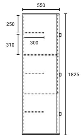
Viking Full 6 Door L720xD550x1825mmH
