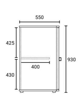
Viking Half 2 Door L720xD550x930mmH
